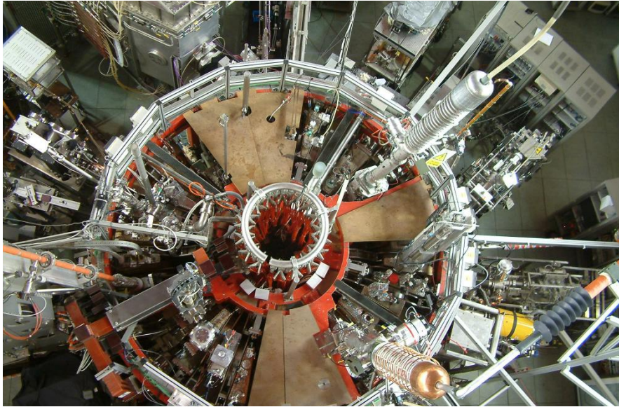
ICTS- LNF: stellarator TJ-II
