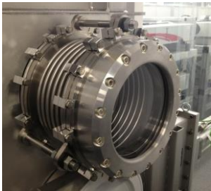
Patent of easy mounting large viewport, with CLPU
