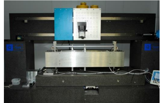
ALBA-NOM (nanometer optical component measuring machine)
