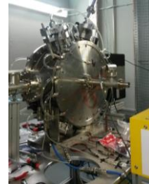
CIEMAT - IFMIF Buncher cavity at ALBA RF lab for High Power Conditioning
