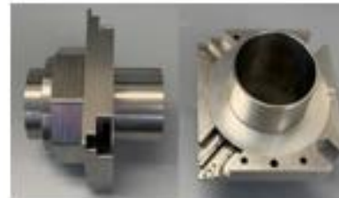
Large Hollow Shaft Design
